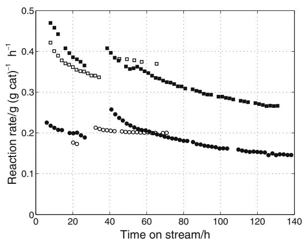
Figure 3. Reaction rates for formation of hydrocarbons at 483 K, 20 bar, and \text{H}_2/\text{CO} = 2.1 (■ = Co/Platelet, □ = \text{Co}/\gamma\text{-Al}_2\text{O}_3 , ● = Co/Fishbone, ○ = \text{Co}/\alpha\text{-Al}_2\text{O}_3 ).
